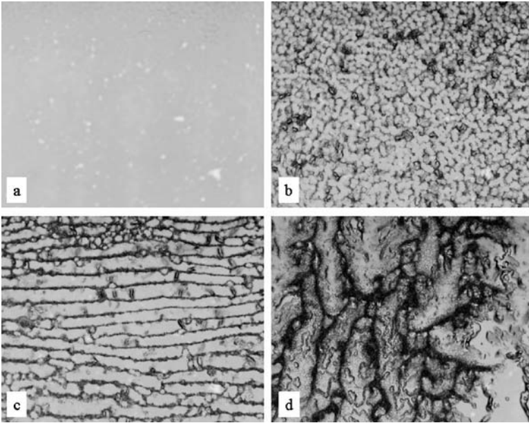
FIGURE 2 Polarized microscopy images of different structures, depending on the cooling rate: (a) colloidal particles are dispersed homogeneously in the isotropic phase; (b) cellular structure: cooling rate = 10^{\circ}\text{C}\cdot\text{min}^{-1} ; (c) stripes : cooling rate = 0.1^{\circ}\text{C}\cdot\text{min}^{-1} , velocity of the interface v \approx 3\mu\text{m}\cdot\text{sec}^{-1} ; (d) root structure: cooling rate = 0.01^{\circ}\text{C}\cdot\text{min}^{-1} , v \approx 0.5\mu\text{m}\cdot\text{sec}^{-1} . Silica particles, R = 0.005\mu\text{m} , concentration \phi = 1\text{ wt\%} . The N-I interface is moving from the top of the pictures downwards. The long side of the images is 1 mm.
