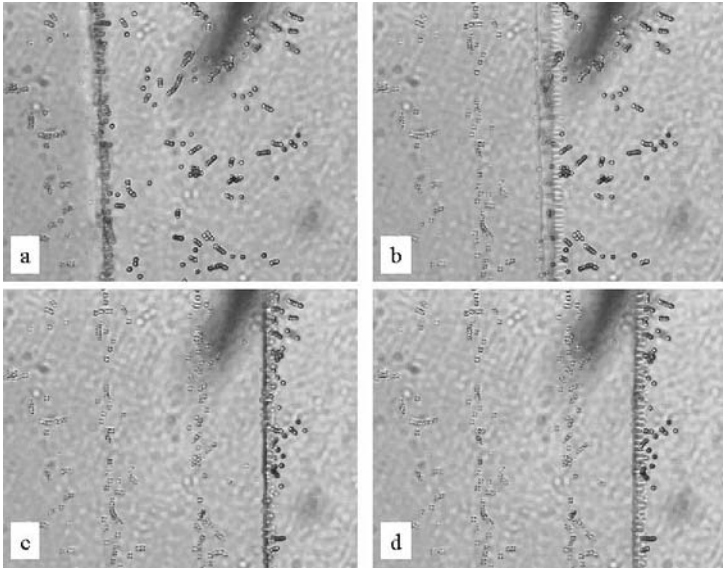
FIGURE 6 Formation of the stripes of particles by the movement of the nematic-isotropic interface and periodic action of an electric field. The nematic phase is on the left size of the pictures.
