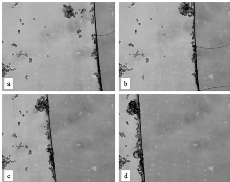
FIGURE 3 Snapshots of the moving nematic-isotropic interface made between parallel polarizers taken with the time interval \Delta t = 6 \text{ min} .
